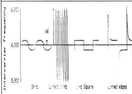
Fig.1: Pre-emphasis
