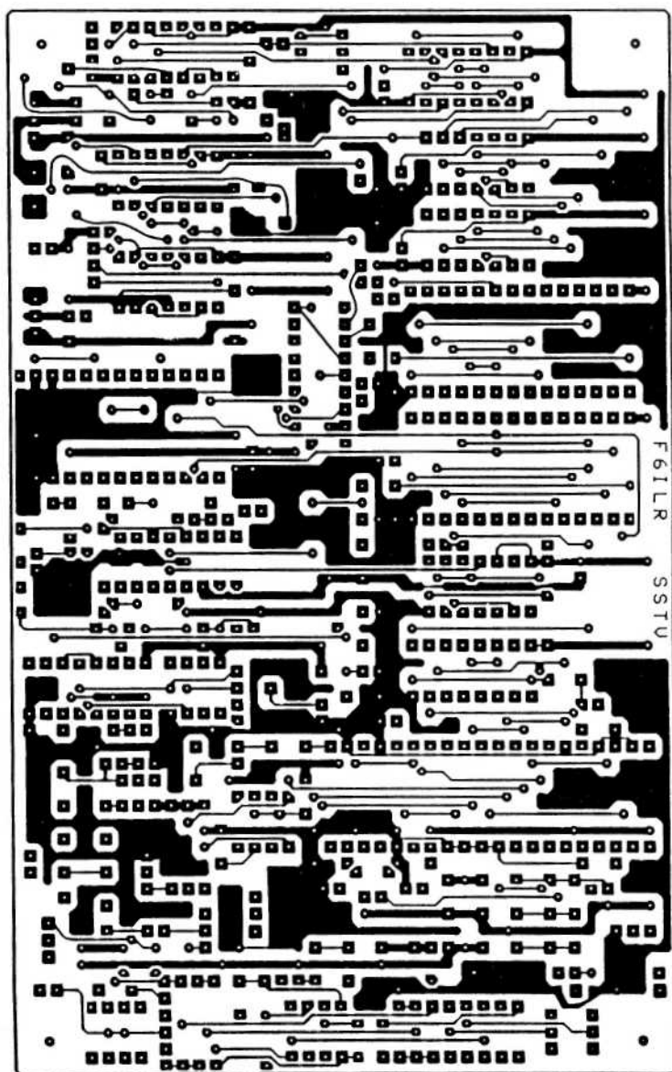
Fig.2a: PCB Layout Track side (actual size)
