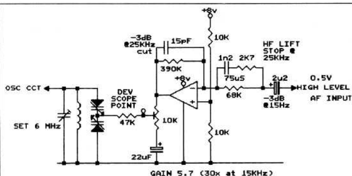
Fig.1: Pre-emphasis
