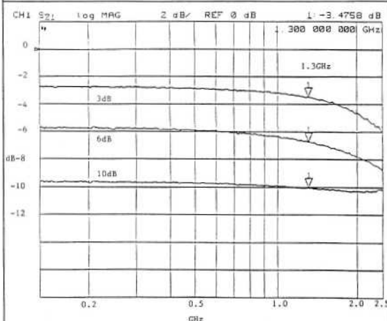
Fig.1: Coaxial Attenuators
