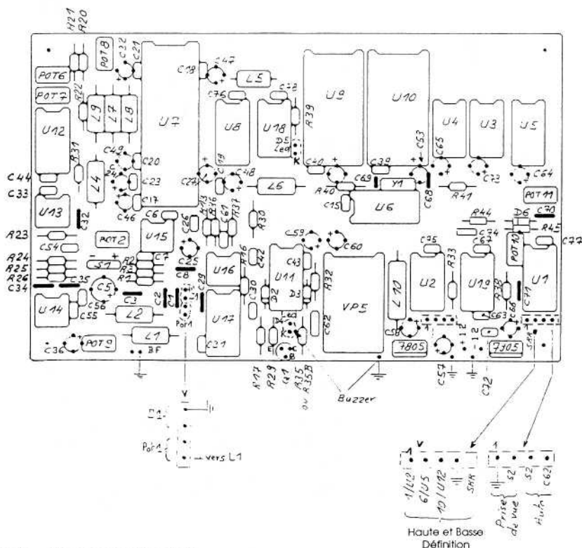
Fig.3: Component Layout
